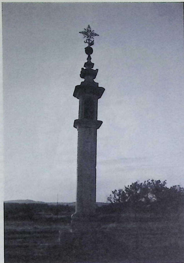
San Roque
